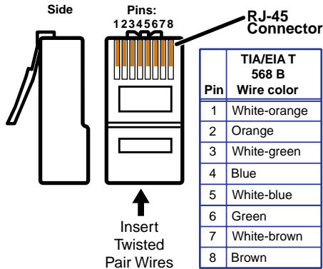
Figure 5. TP Cable Termination
